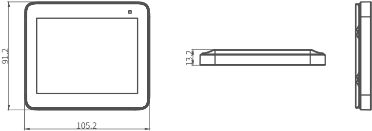
TECHNICAL DRAWINGS (mm)
